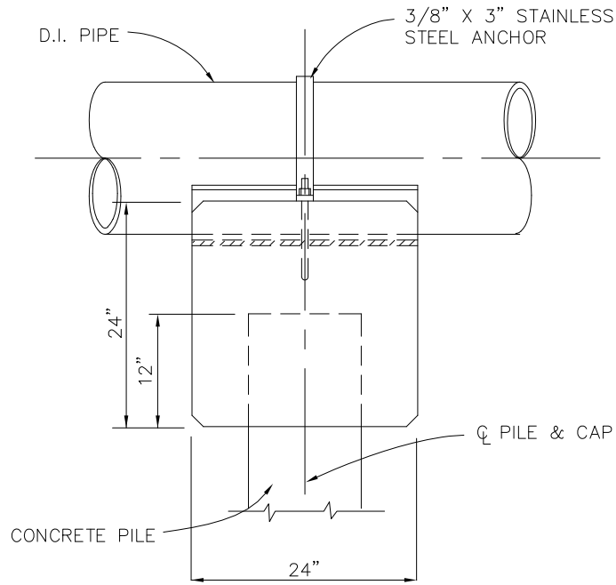
VIEW C-C
